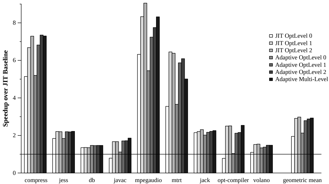
Figure 6: Steady-state performance
